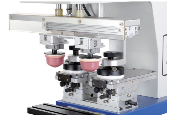
▲ 油盅结构 Ink Cup Structure
